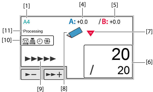
[Processing] screen
